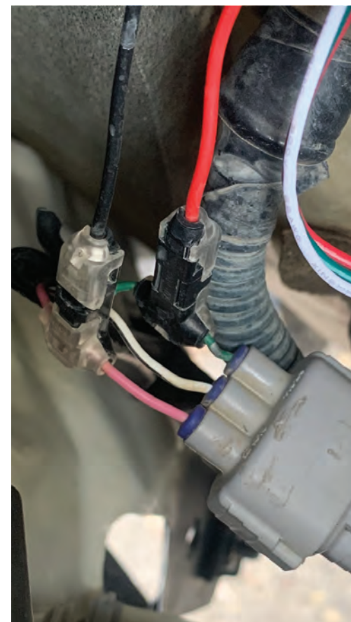
Wiring Example B
